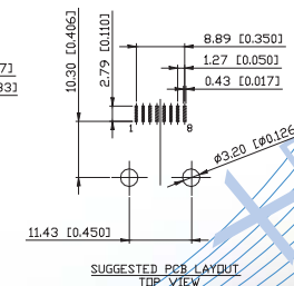
SUGGESTED PCB LAYOUT TOP VIEW
