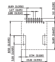
SUGGESTED PCB LAYOUT TOP VIEW
