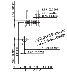
SUGGESTED PCB LAYOUT TOP VIEW
