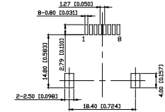
SUGGESTED PCB LAYOUT TOP VIEW
