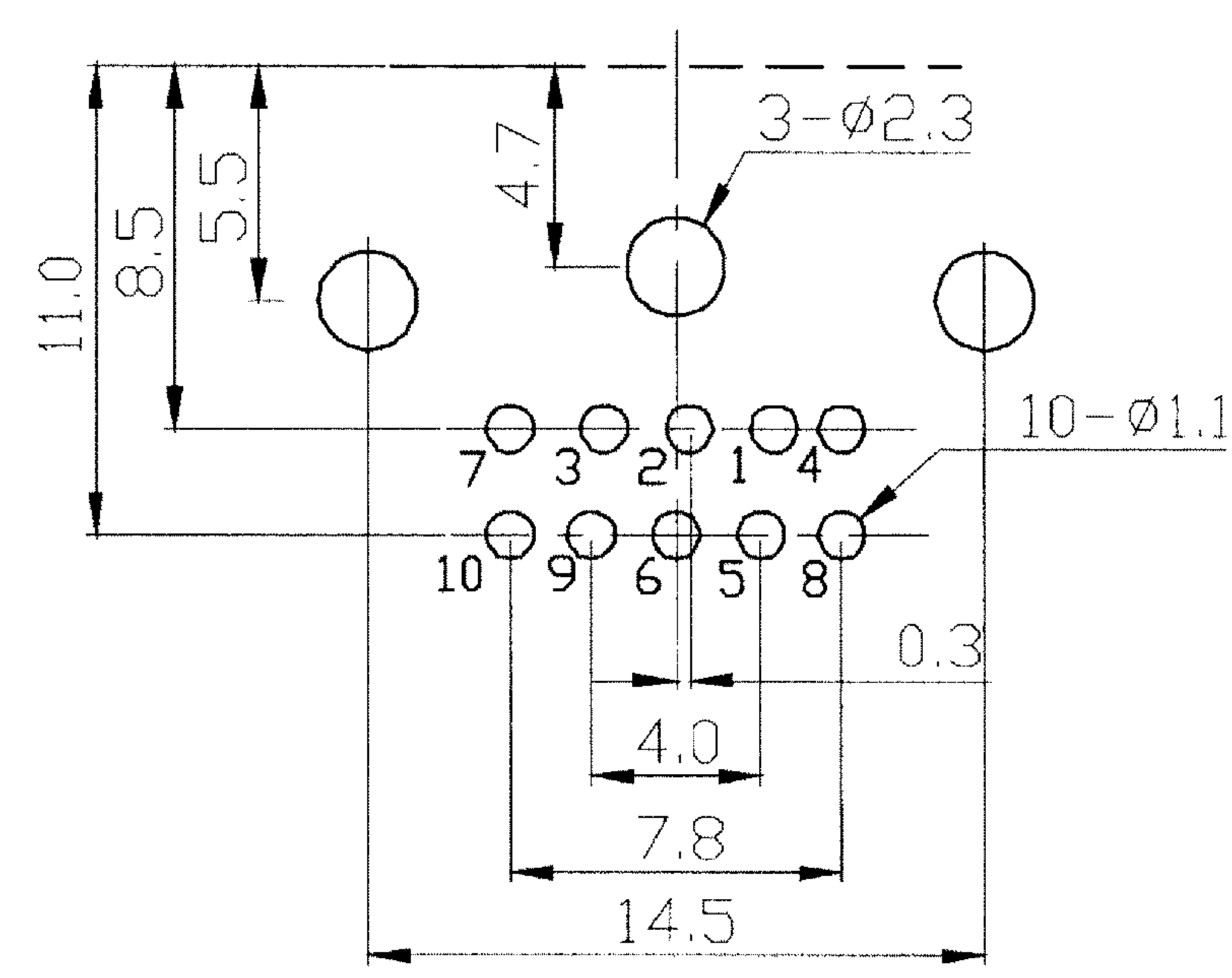
P.C.B. LAYOUT (BOTTOM VIEW)
