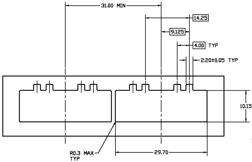
RECOMMENDED BEZEL CUT-OUT SINGLE SIDED APPLICATIONS
