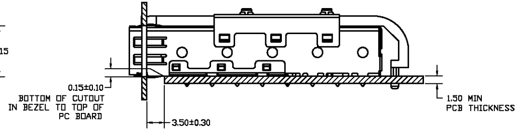
MOUNTED ON PC BOARD SHOWN THRU RECOMMENDED BEZEL
