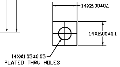
DETAIL B SCALE 4:1
