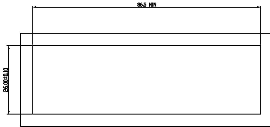
BEZEL CUT-OUT CENTER SPACING DETAIL BEZEL THICKNESS:0.8-2.6
