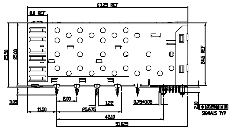
PART NUMBER SFP026BL
