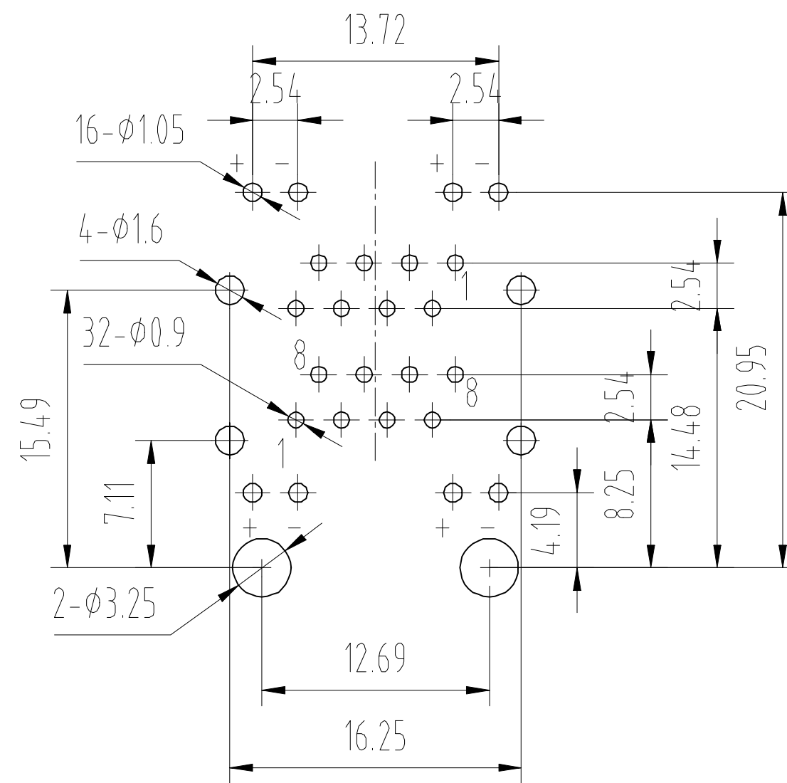
PC Board Layout Component Side Shown
