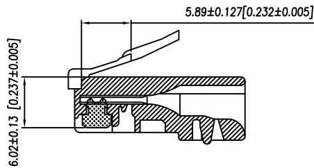
RECOMMENED PLUG DIMENSION
