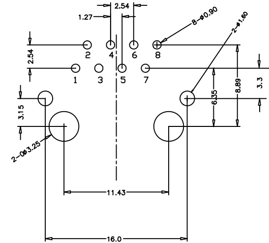
Suggested PCB Layout (Component Side Shown)
