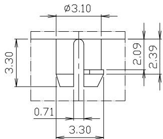
DETAIL X
