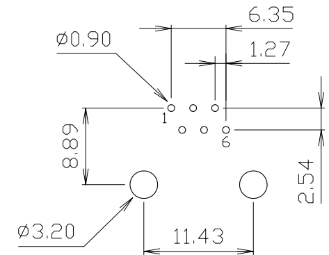
PC Board Layout Ref.
