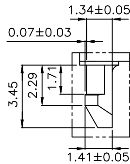
DETAIL X
