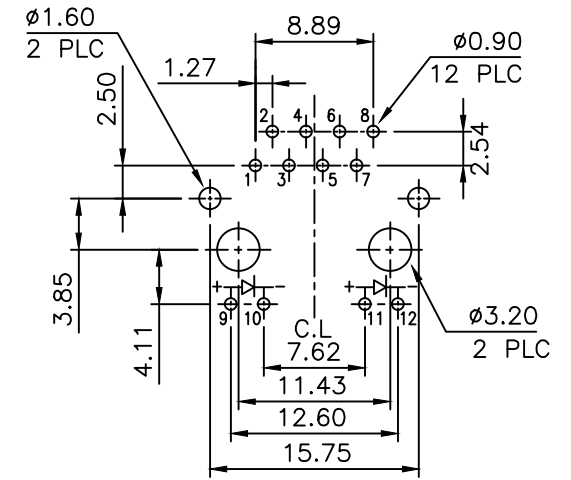
PCB Layout
