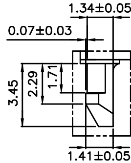
DETAIL X
