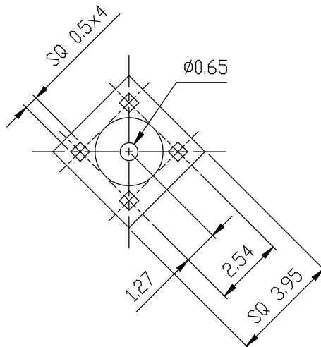
Recommend Mounting Hole
