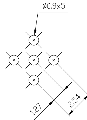
Recommend Mounting Hole
