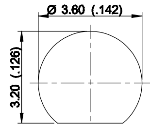
MOUNTING HOLE
