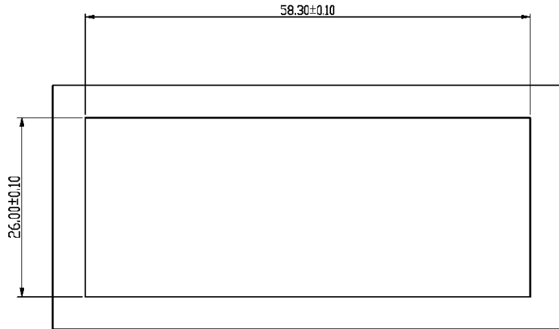
BEZEL CUT-OUT CENTER SPACING DETAIL BEZEL THICKNESS:0.8-2.6
