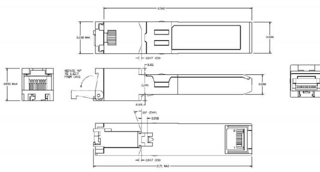
Figure2. Mechanical Specifications
