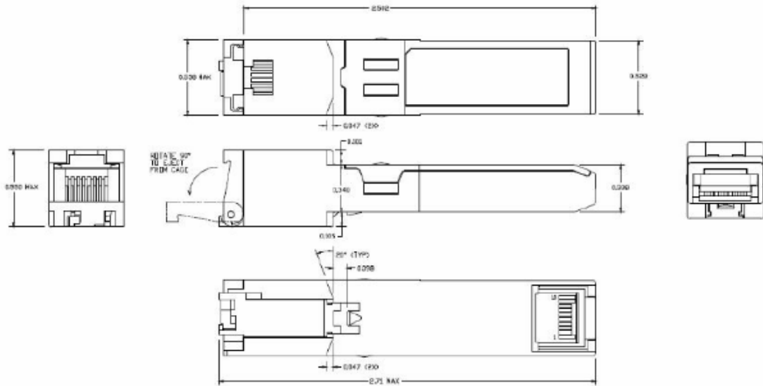
Figure2. XSFP-SPT-PE-T1 mechanical dimensions
