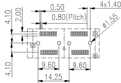
CONNECTOR LAYOUT
